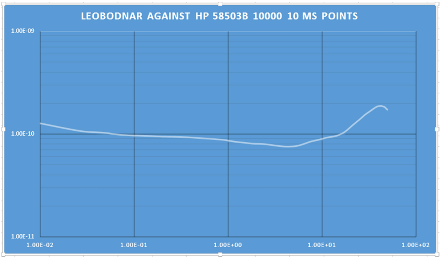
Allan Deviation for Leobodnar GPSDO against HP58503B GPSDO 10000 10ms points
