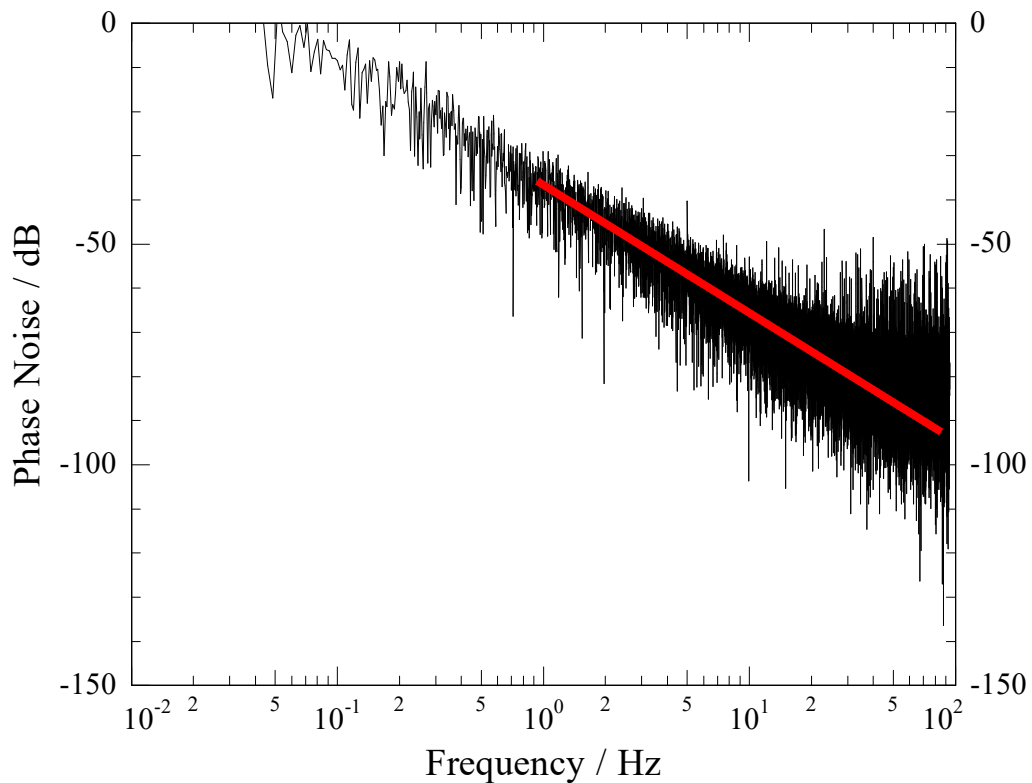
65000 5.33ms points at 499MHz
