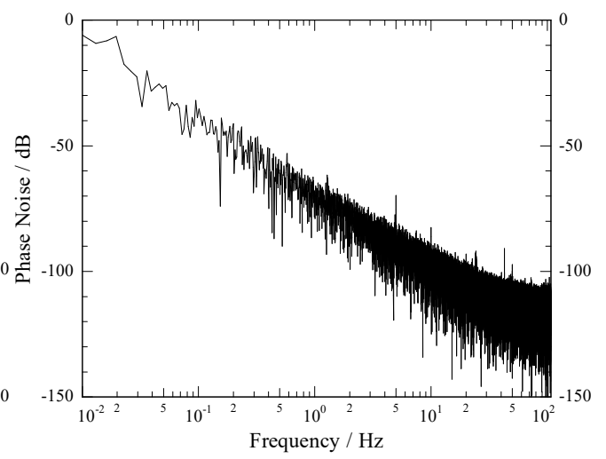
65000 4.67ms points at 10MHz
