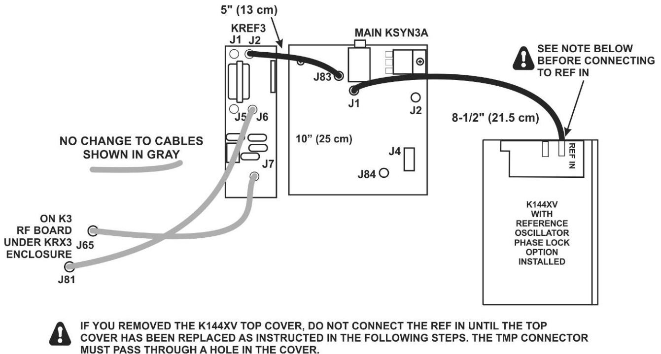
Figure 12. Coaxial Cable Connections for K3 with no KRX3 Sub Receiver.
