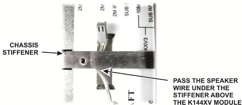
Figure 16. Routing the Speaker Wire Under the Chassis Stiffener.
